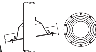
PIPE BOOT INSTALLATION
